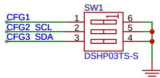
Output Voltage Selection Switches
