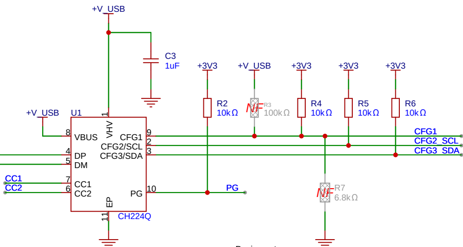
USB PD Controller
